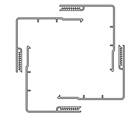
4" Wrap fits from 3-1/4" square to 4-3/8" square posts.
