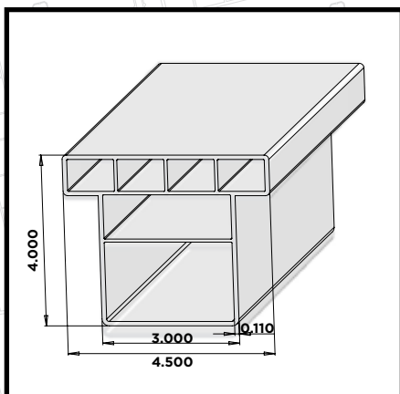
4-1/2" GORILLA® RAIL
