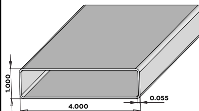
1" X 4" UTILITY PICKETS
