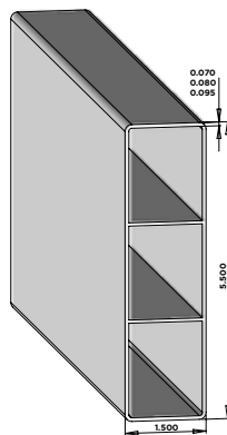
1-1/2" X 5-1/2" RIBBED RAIL (UTILITY & UTILITY VALUE)
