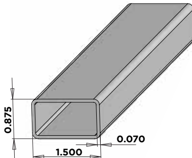
7/8" X 1-1/2" STANDARD PICKETS
