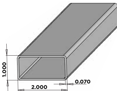
1" X 2" STANDARD PICKETS
