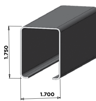
2" STEEL INSERT - 2" POCKET RAIL
