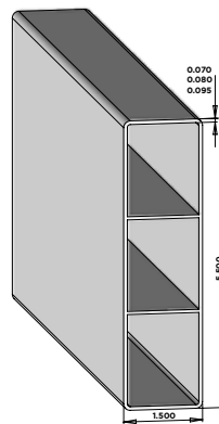
1-1/2" X 5-1/2" RIBBED RAIL
