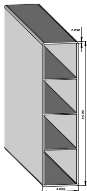
2" X 8" RIBBED RAIL
