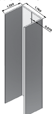
1-1/2 GORILLA® POST INSERT
