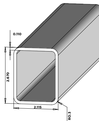
2-1/8" X 2-3/4" STANDARD RAIL
