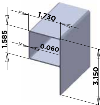
2" X 3-1/2" & T-RAIL
