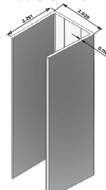
1-3/4 GORILLA® FENCE U-CHANNEL
