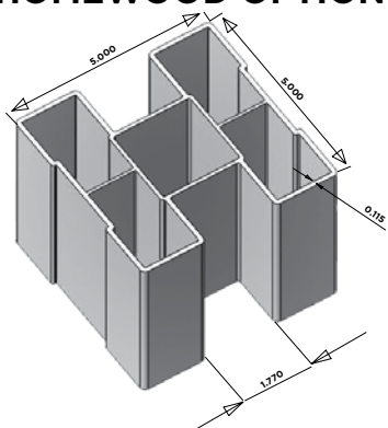
5" X 5" GORILLA® H-POST
