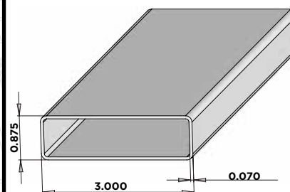
7/8" X 3" STANDARD PICKETS
