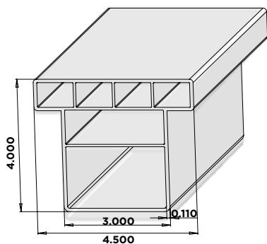
4-1/2" GORILLA® RAIL
