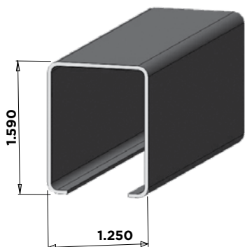
1-1/2" STEEL INSERT - POCKET RAIL
