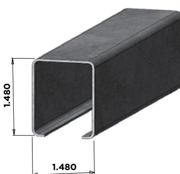
1-3/4" STEEL INSERT - POCKET RAIL
