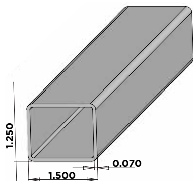
1-1/4" X 1-1/2" STANDARD PICKETS
