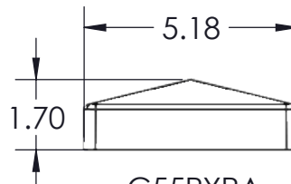
C55PYRA 5" x 5" External Pyramid Post Cap
