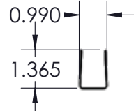
F83U 7/8" x 58-3/4" Trim Channel
