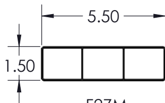
F27M 1½" x 5½" Co-Ex Utility Value Rail
