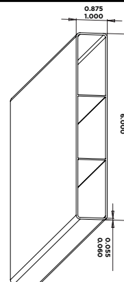
7/8" X 6" RIBBED STANDARD
