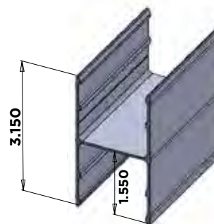
H-RAIL - ALUMINUM INSERT
