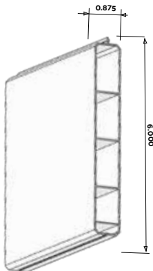
7/8" X 6" GORILLA® LOCKING PICKET
