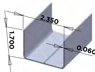
2-1/8" X 2-3/4" DOWN - ALUMINUM INSERT
